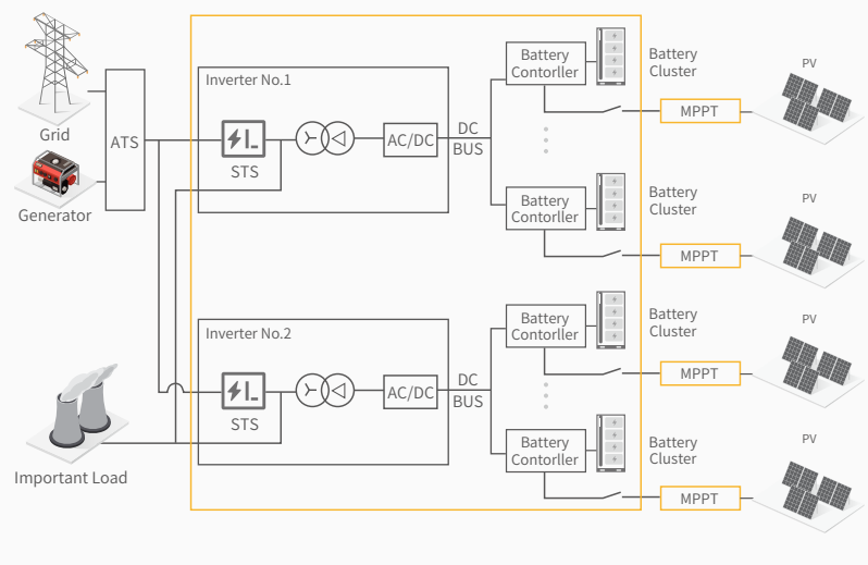
System block diagram
